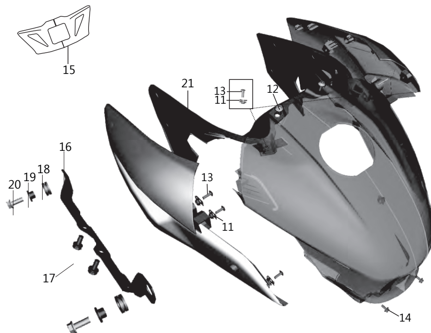
RH Mounting
